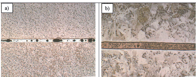
Fig. 2. Macrostructure of induction brazed joint of titanium Grade 2 using Ag 272 (a) and Cu 099 filler metal and F60T flux.
