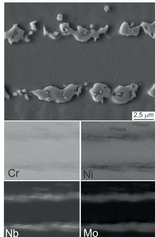
Fig. 2. The maps of particular elements distribution obtained by SEM/EDS
