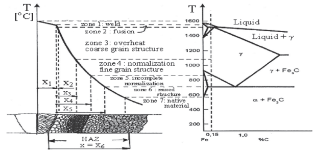
Fig. 1. The example of HAZ structure for carbon steel containing 0.15% C, see [1]
