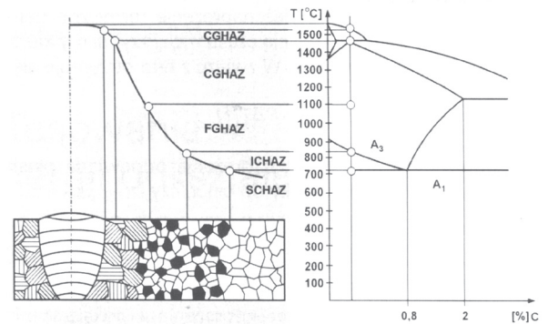
Fig. 2. Distribution of structural areas of HAZ for low alloy steel as a function of temperature, in relation to the iron-carbon phase equilibrium [10]
