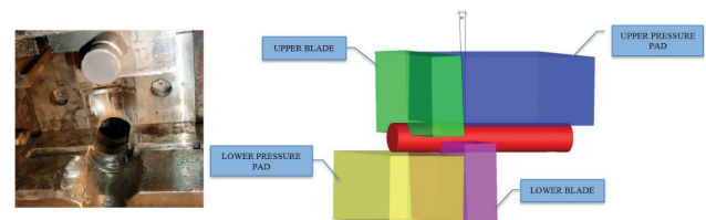
Fig. 2. Scheme of the cutting method: a) image of the shearing machine and b) numerical model of the cutting process after changes – introduced blade inclination
