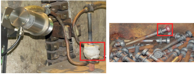
Fig. 7. Local induction heating of a forging
