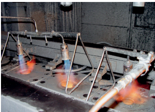
Fig. 13. Heating up the tools with gas burners
