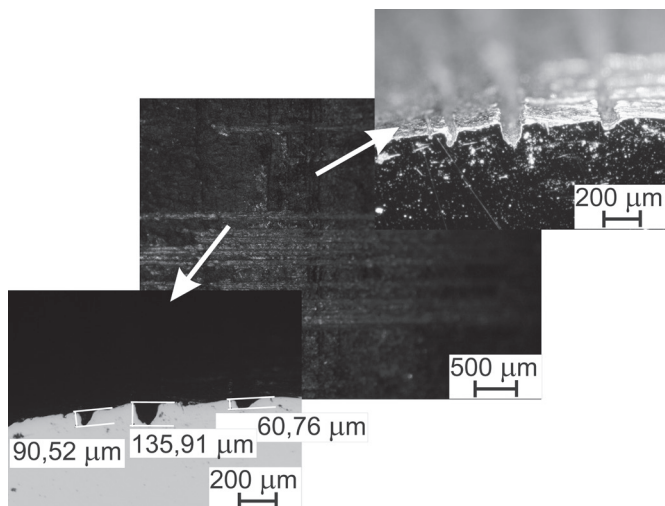
Fig. 8. Macroscopic and microscopic views of fissures and cracks on
