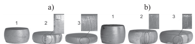
Fig. 2. A general view of 16.5 mm-diameter 20MnB4 steel specimens after the cold upsetting process: a) specimens with a height of 1.5 d; b) specimens with a height of 2.0 d; 1 – relative plastic strain of 50%; 2 – relative plastic strain of 66%; 3 – relative plastic strain 75%
