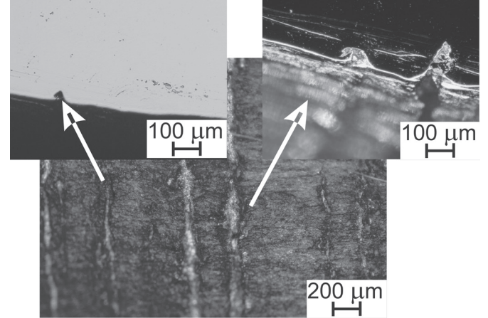
Fig. 9. Macroscopic and microscopic views of fractures and cracks on the 2.0 d-initial length 20MnB4 steel specimen – relative strain 75 %
