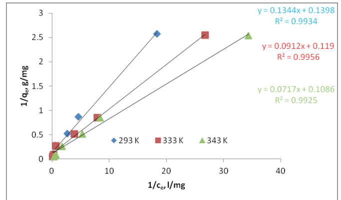
Fig. 3. Langmuir adsorption isotherm for the system of waste foundry molding sand/Cu (II) ions
