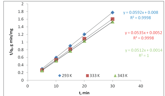
Fig. 6. Linearized shape of pseudo second order kinetic model for system of waste foundry molding sand /Cu (II) ions
