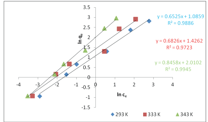
Fig. 2. Freundlich adsorption isotherm for the system of waste foundry molding sand/Cu (II) ions
