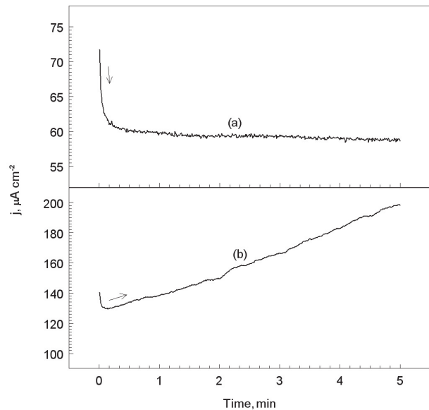
Fig. 7. Chronoamperometric curves obtained at 25°C in Ringer's solution for uncoated X46Cr13 steel at: (a) -330, and (b) 50 mV
