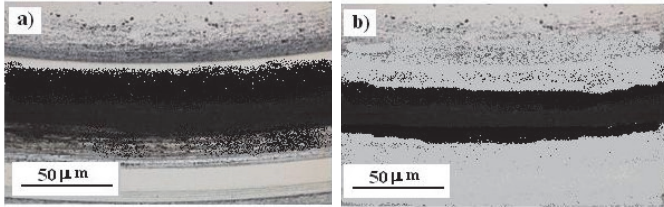
Fig. 2. Wear tracks on: (a) uncoated, and (b) DLC coated X46Cr13 steel
