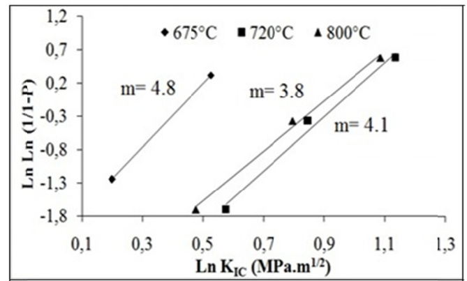
Fig. 7. Weibull plots for indentation fracture toughness data
