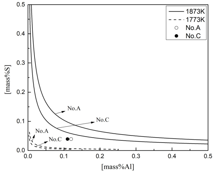
Fig. 8. Equilibrium phase diagram of MgS-MgO·Al 2 O 3 reaction at 1,873K and 1,773K
