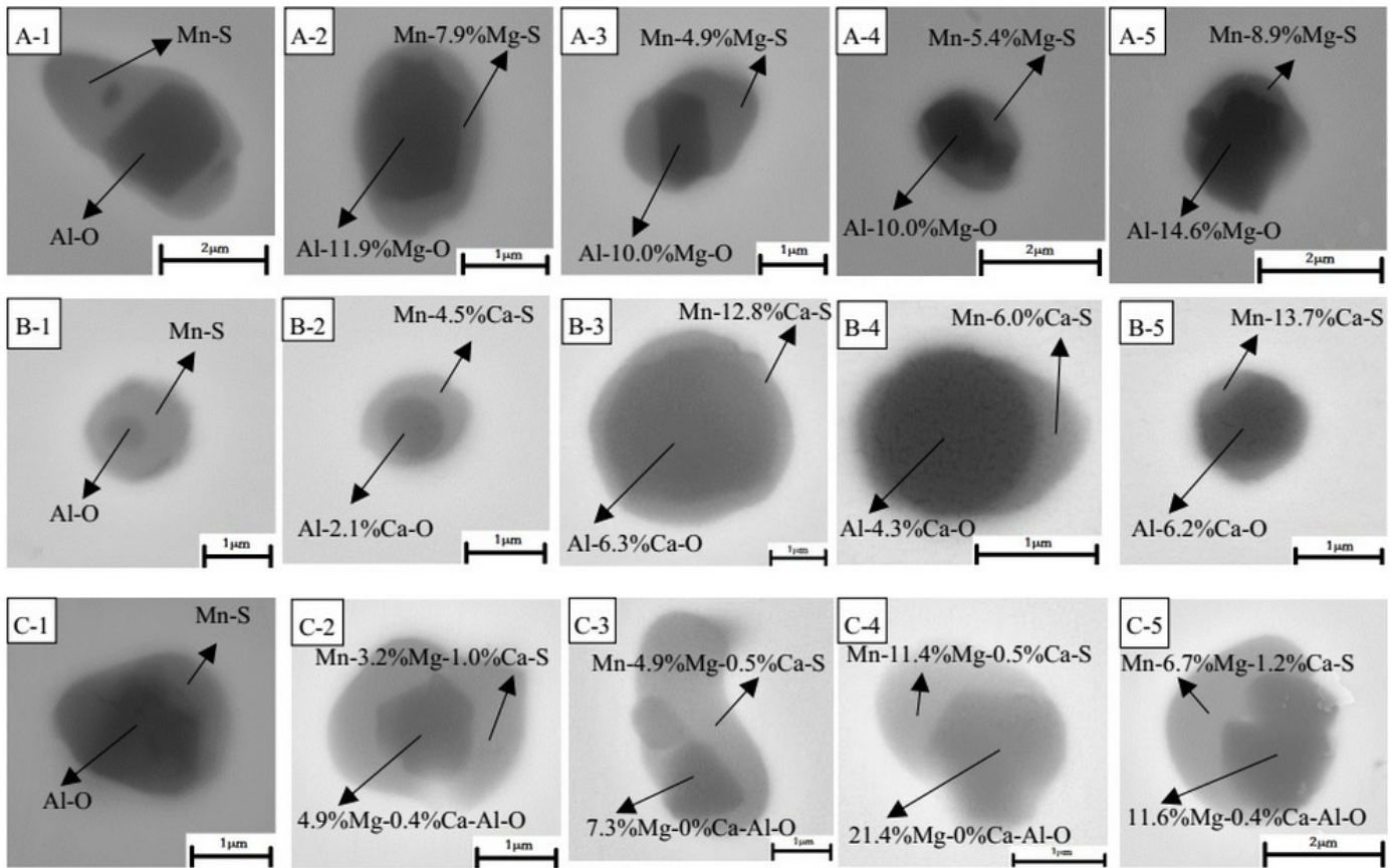
Fig. 2. Morphology and composition of typical inclusions of the samples. A, B, and C indicate melt numbers; 1, 2, 3, 4, and 5 denote samples 1#, 2#, 3#, 4#, and 5#, respectively
