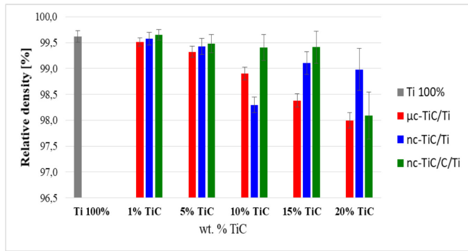
Fig. 7. Comparison of relative density values of TiC/Ti composites with different TiC content
