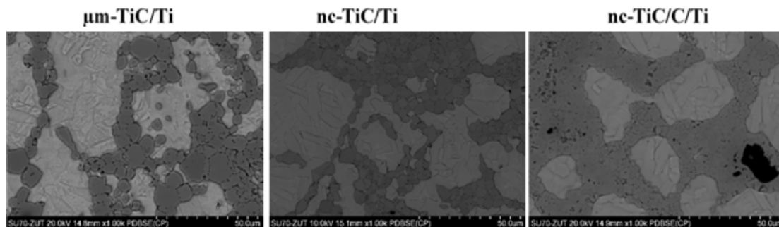
Fig. 6. SEM images of electropolished TiMMCs samples containing 20 wt % of TiC
