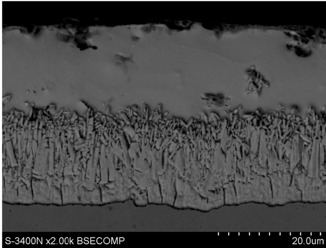
Fig. 1. Coat cross-section (SEM) microstructure for galvanized C42D steel wire rod
