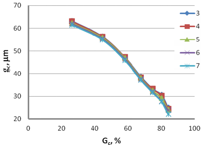
Fig. 5. Variation in zinc coat thickness g as a function of the total reduction
