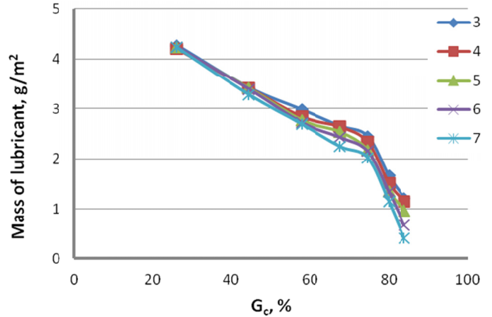
Fig. 3. Variation in lubricant mass on the wire surface at an angle of \alpha = 3-7^\circ as a function of the total reduction
