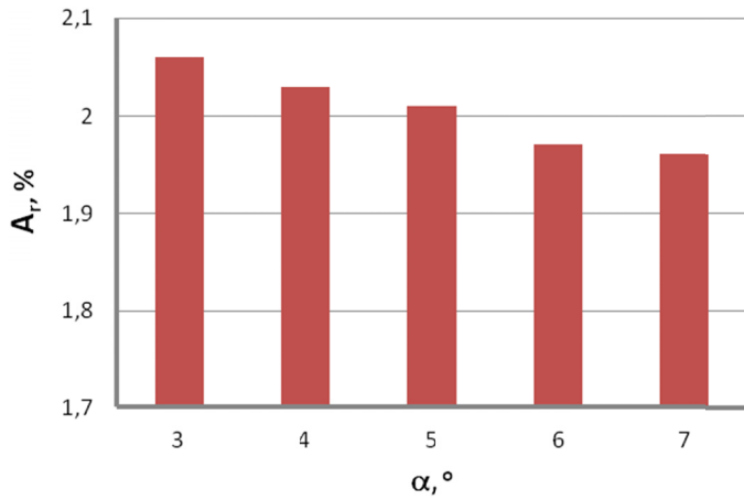
Fig. 8. Variation in uniform elongation, A_r , as a function of drawing angle \alpha
