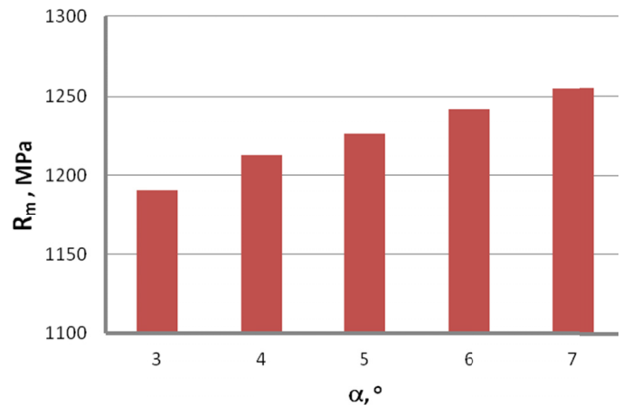
Fig. 7. Variation in ultimate tensile strength, R_m , as a function of drawing angle \alpha
