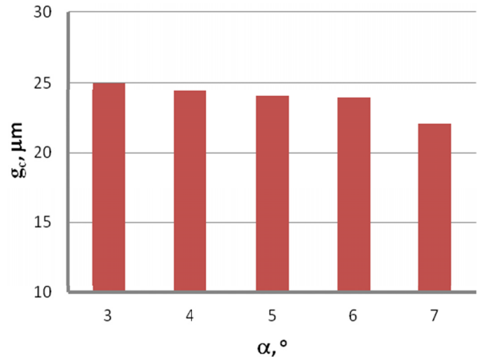
Fig. 4. The effect of drawing angle \alpha on the zinc coat thickness, g_c , for 2.2 mm-diameter wires
