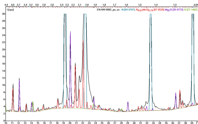
Fig. 3. Diffraction pattern of EN AW-6082 alloy. Intensity scale factor = 100:1
