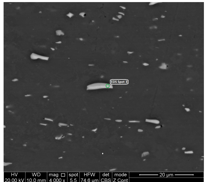
Fig. 9. Scanning electron microscope image of EN AW-8011 alloy
