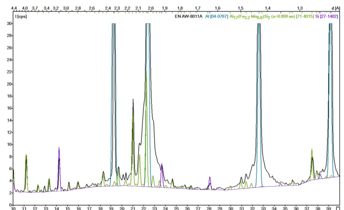
Fig. 4. Diffraction pattern of EN AW-8011 alloy. Intensity scale factor = 80:1
