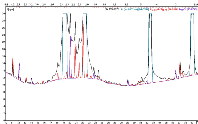
Fig. 1. Diffraction pattern of EN AW-7075 alloy. Intensity scale factor = 40:1
