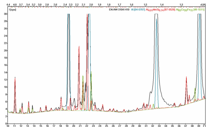
Fig. 2. Diffraction pattern of EN AW-3104 alloy. Intensity scale factor = 20:1
