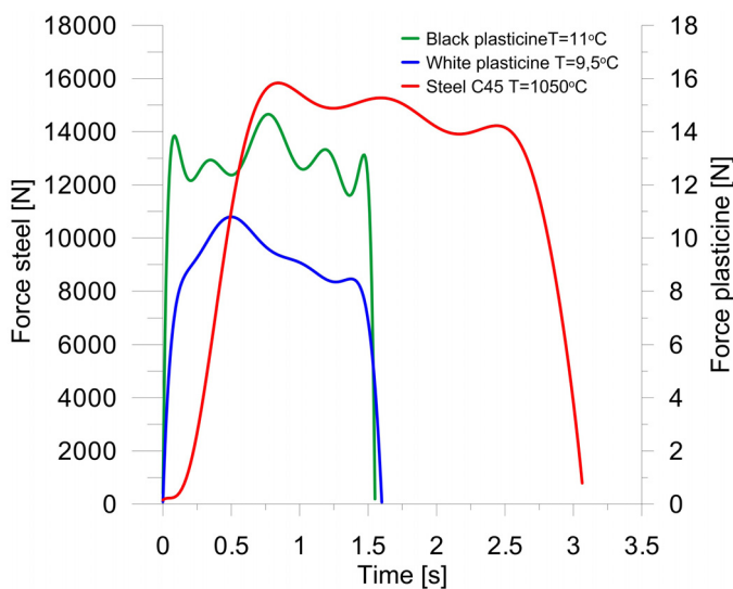
Fig. 10. Progression of the forming forces
