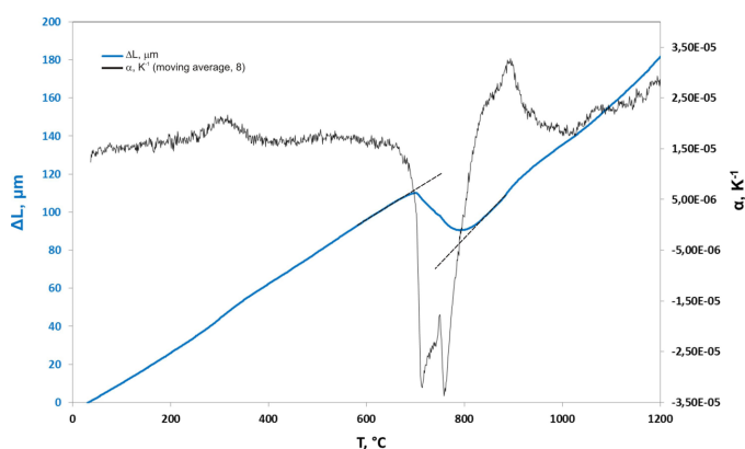
Fig. 2. Dilatometric curve with the corresponding curve of thermal expansion coefficient changes for the tested cast steel, recorded during heating with a 0.08^\circ\text{C/s} rate
