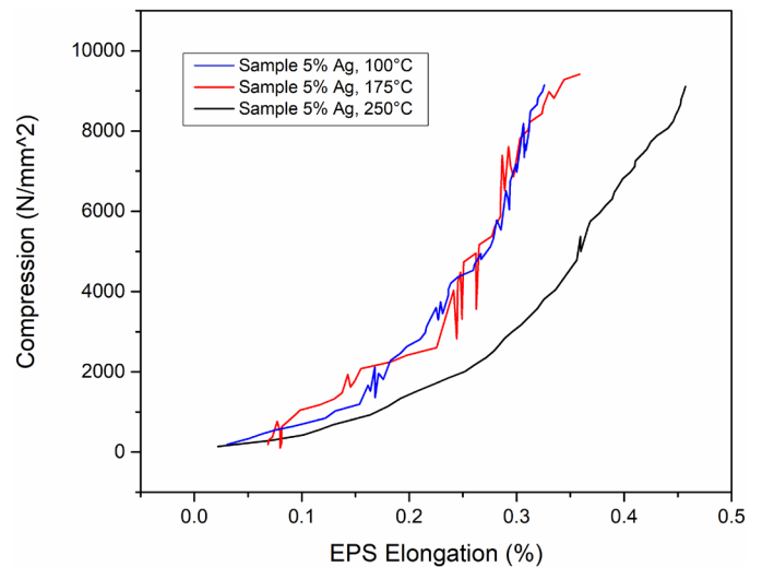
Fig. 6. Compressive strength values for different annealing temperatures and as a function of the silver content therein
