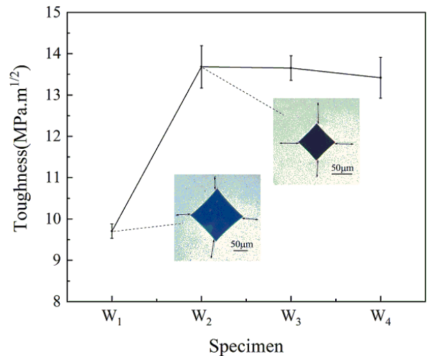
Fig. 4. Fracture toughness of specimens W 1 -W 4
